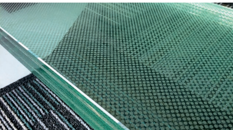
ABOVE: Satin finish non-slip treatment on triple laminate glass stair treads.
